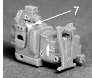
Remove parts from frame and engine as shown
