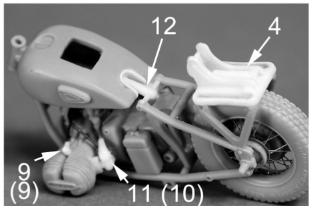
Drill hole in tank to receive part 12
