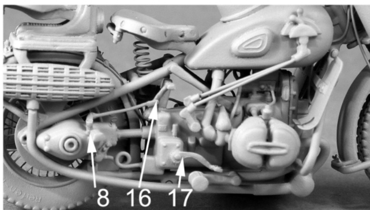
Remove levers from kit handle bars and fit as shown
